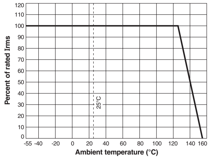
Imax Derating
